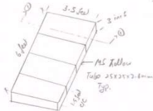
Frame for Table Top
