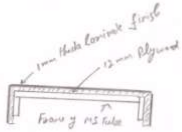
Section 1-1
