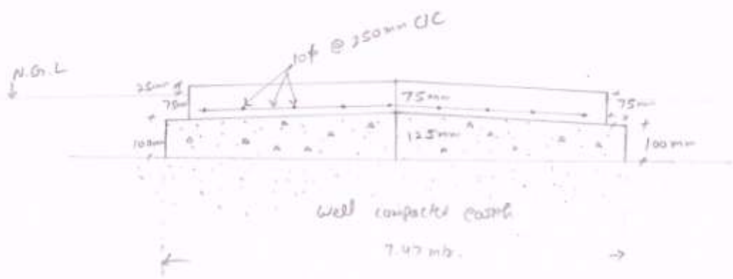
Section 1-1
